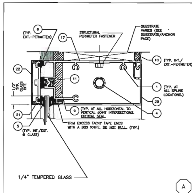
HEAD
