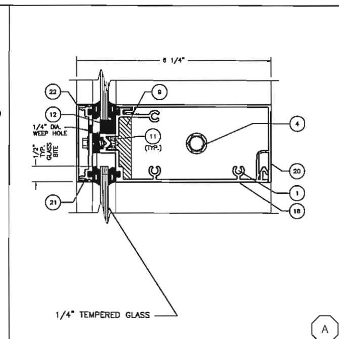
HORIZONTAL
