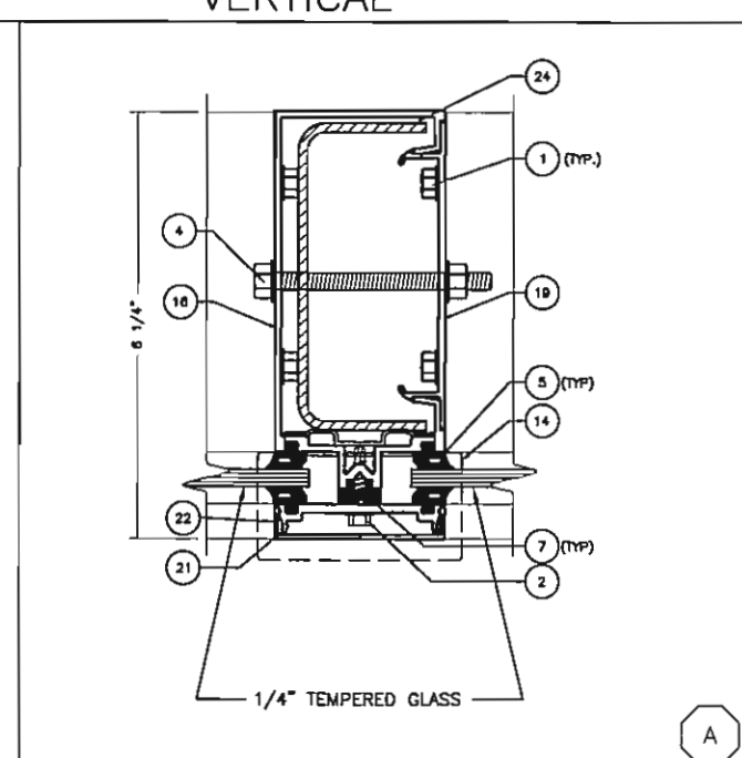
VERTICAL
