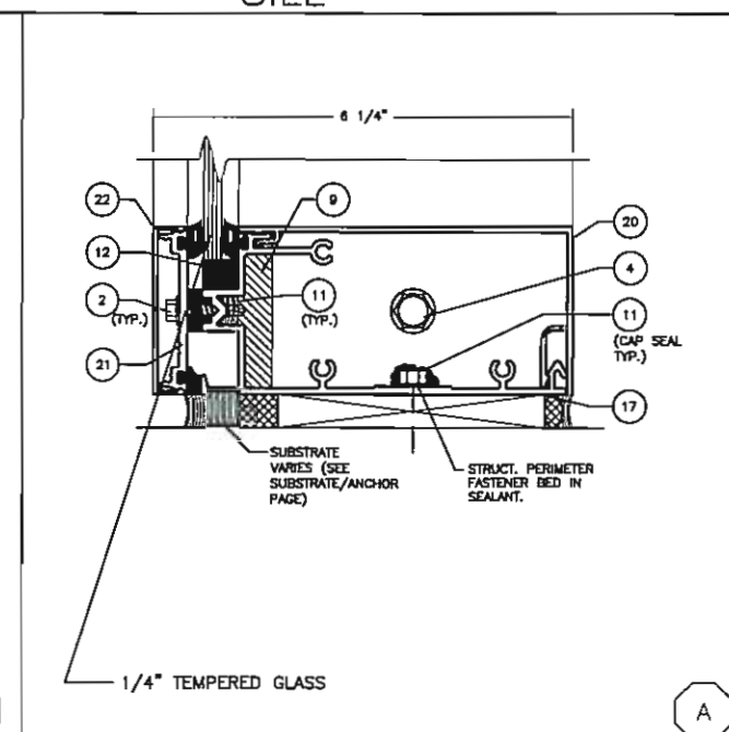
SILL
