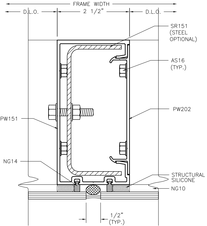
B.G. MULLION W/ SR151 1:2
