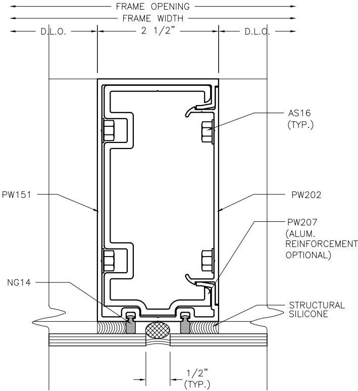
B.G. MULLION W/ SPLICE SLEEVE 1:2
