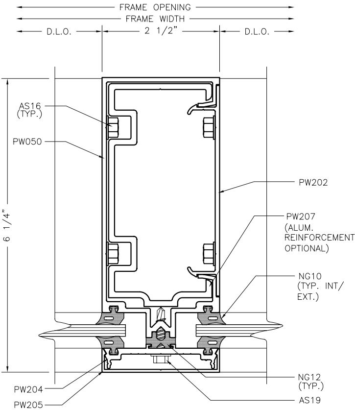
VERTICAL MULLION W/ SPLICE SLEEVE
