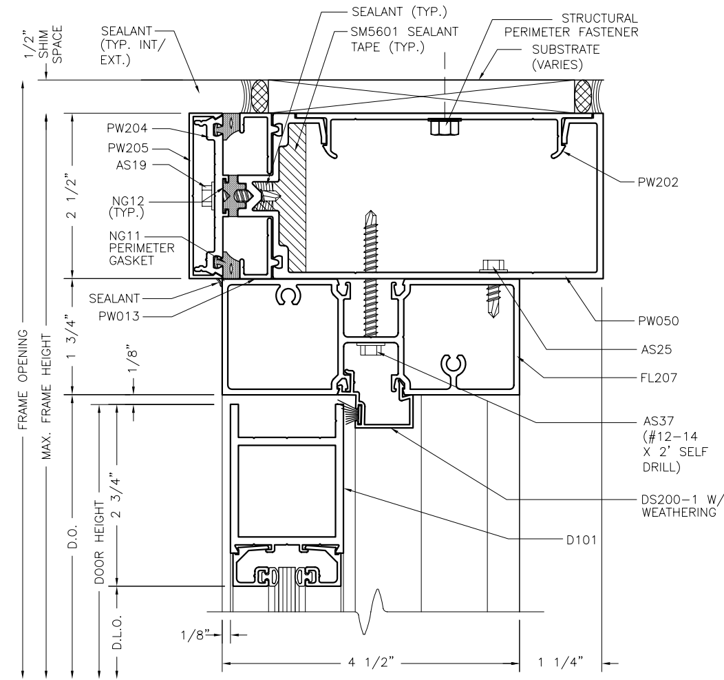
DOOR HEADER FOR SURFACE CLOSER
