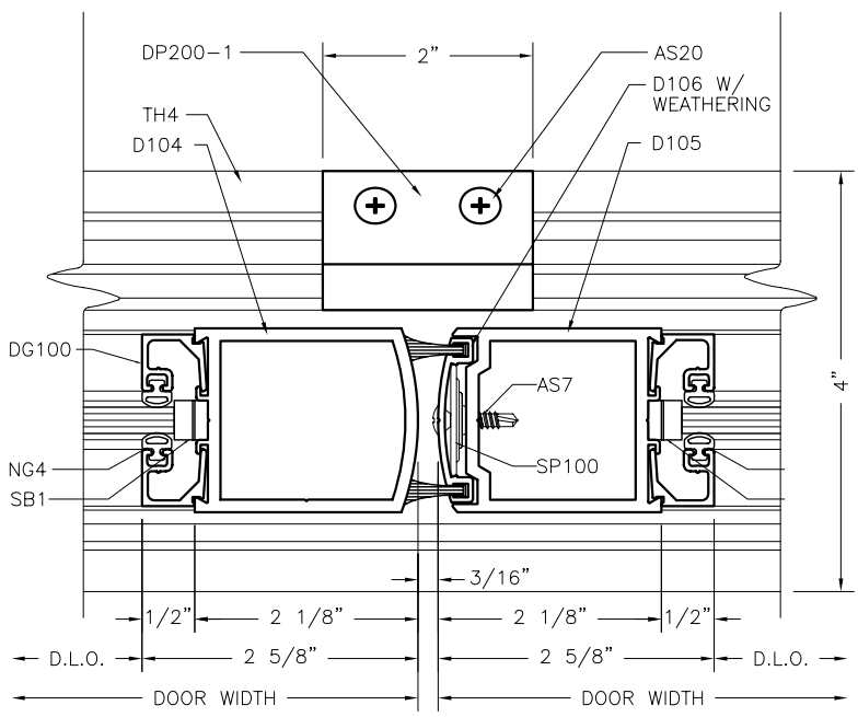
MEETING STILES 1:2
