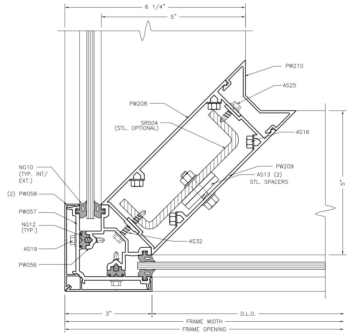
90° CORNER WITH SR504 1:2
