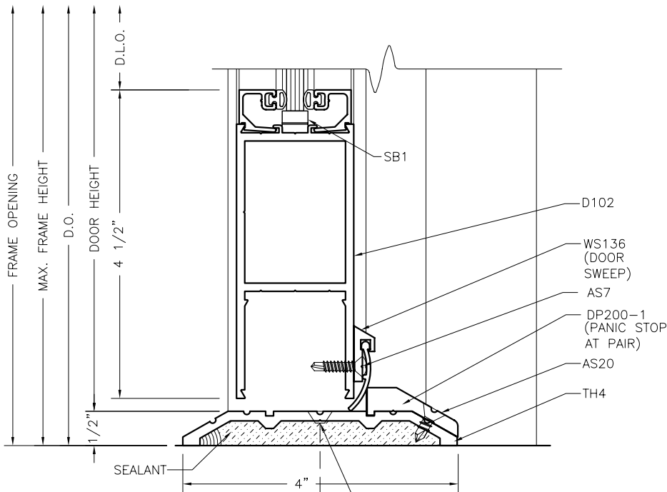
THRESHOLD
