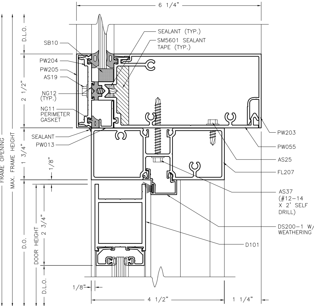
DOOR FRAME HEADER FOR SURFACE CLOSER
