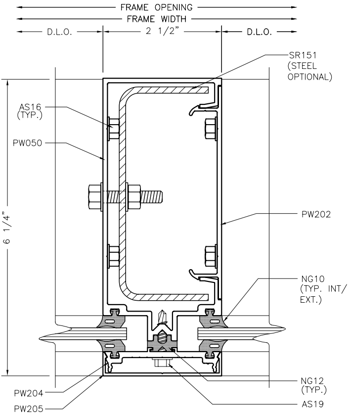
VERTICAL MULLION W/ SR151
