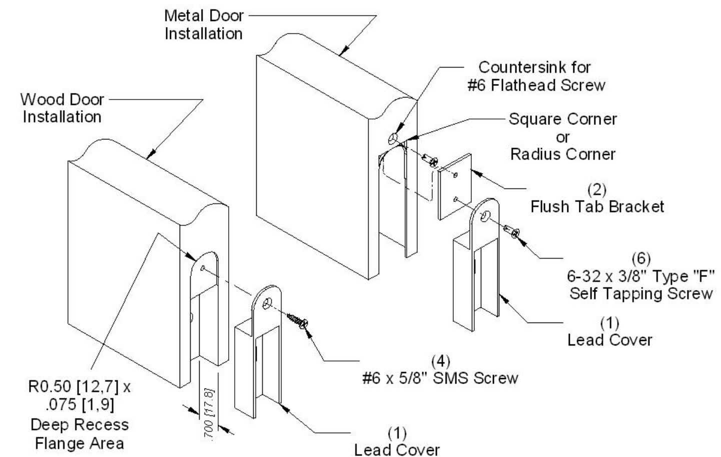
Figure 3 Note: Routing is generally performed into the edge of the door (as shown) but this can be reversed with the routing being done into the frame.
