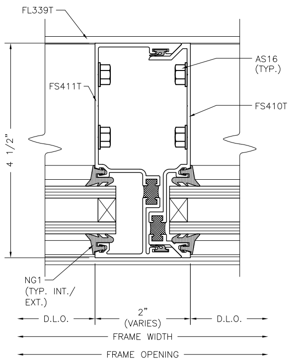
EXPANSION MULLION 1:2
