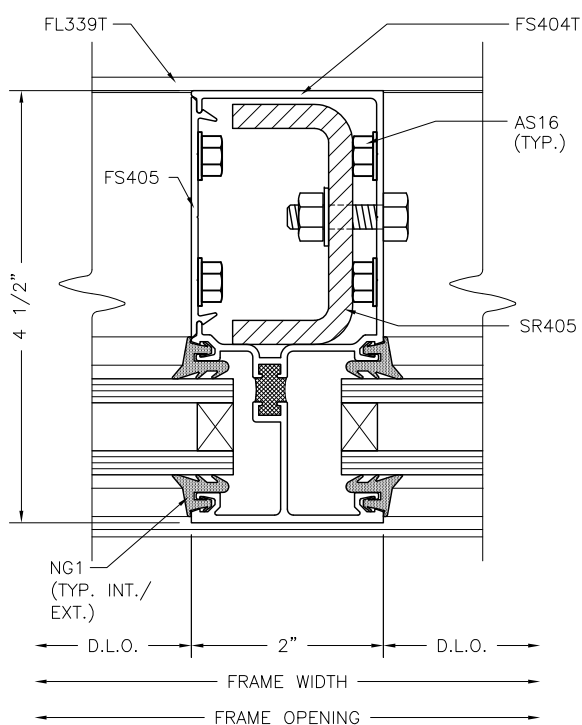
VERTICAL MULLION WITH HEAVY STEEL 1:2
