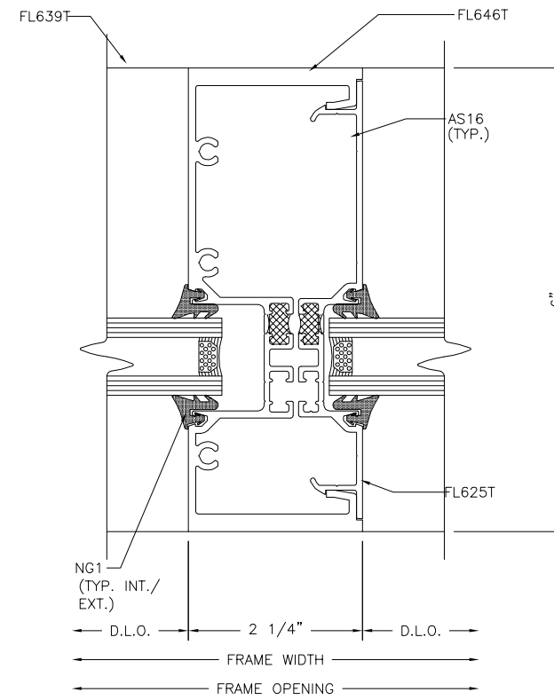
HEAVY VERTICAL
