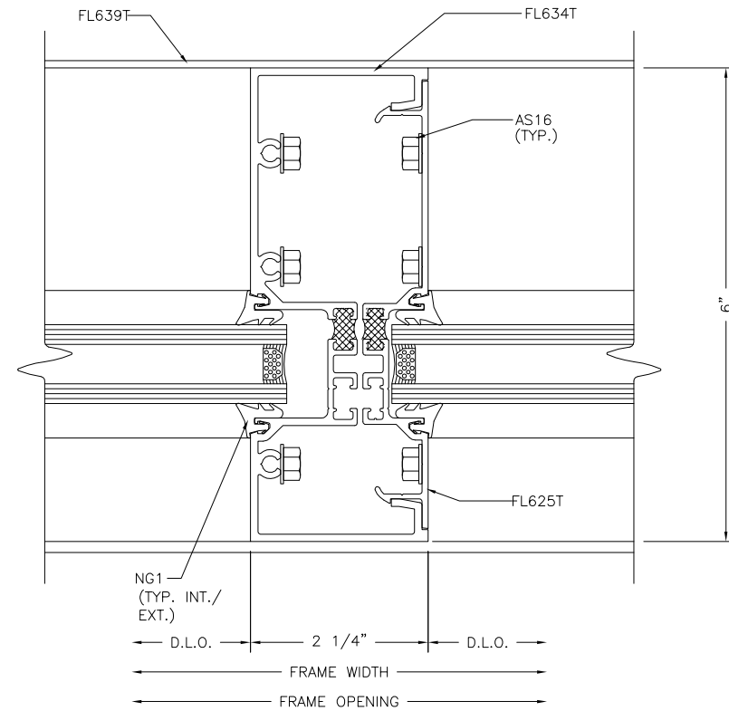
VERTICAL MULLION
