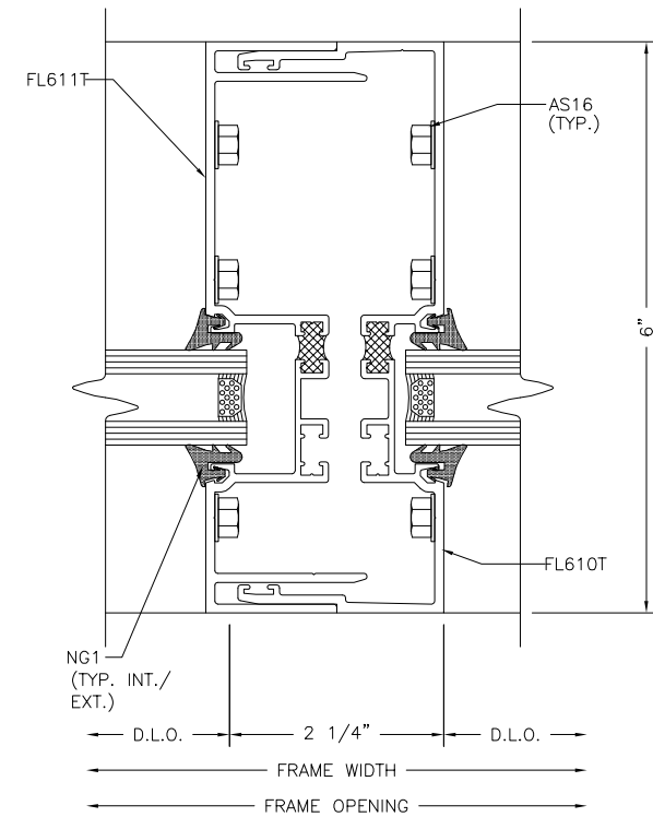
EXPANSION MULLION
