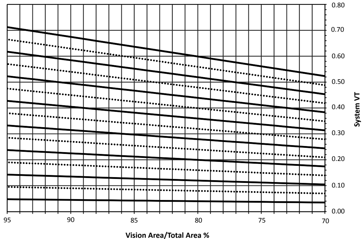
System VT vs. Percentage of Vision Area
