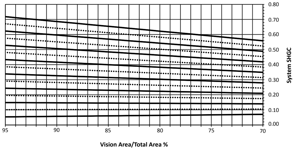
System SHGC vs. Percentage of Vision Area
