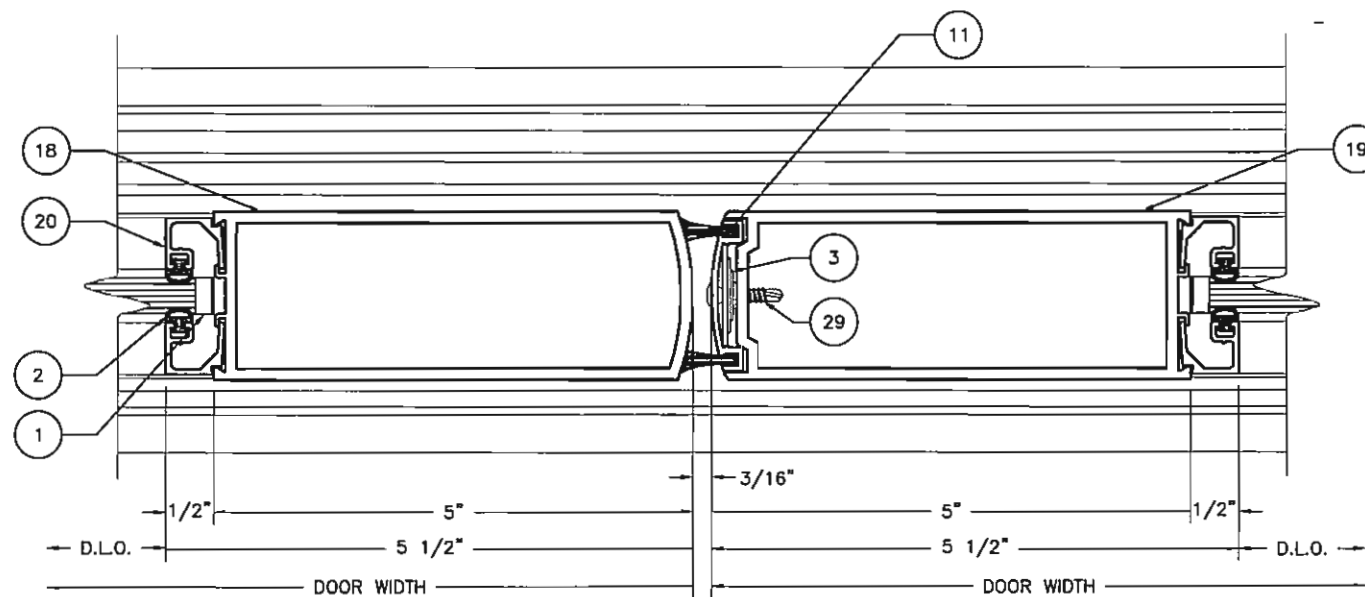
14 WS MEETING STILES 11 SCALE: 1:2
