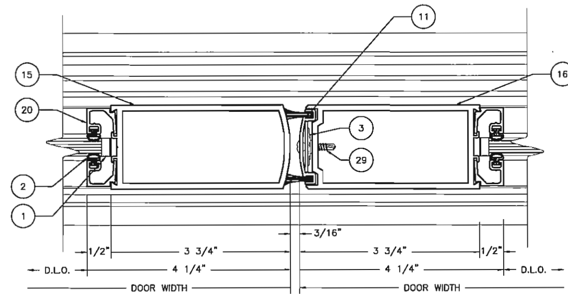
13 MS MEETING STILES 11 SCALE: 1:2
