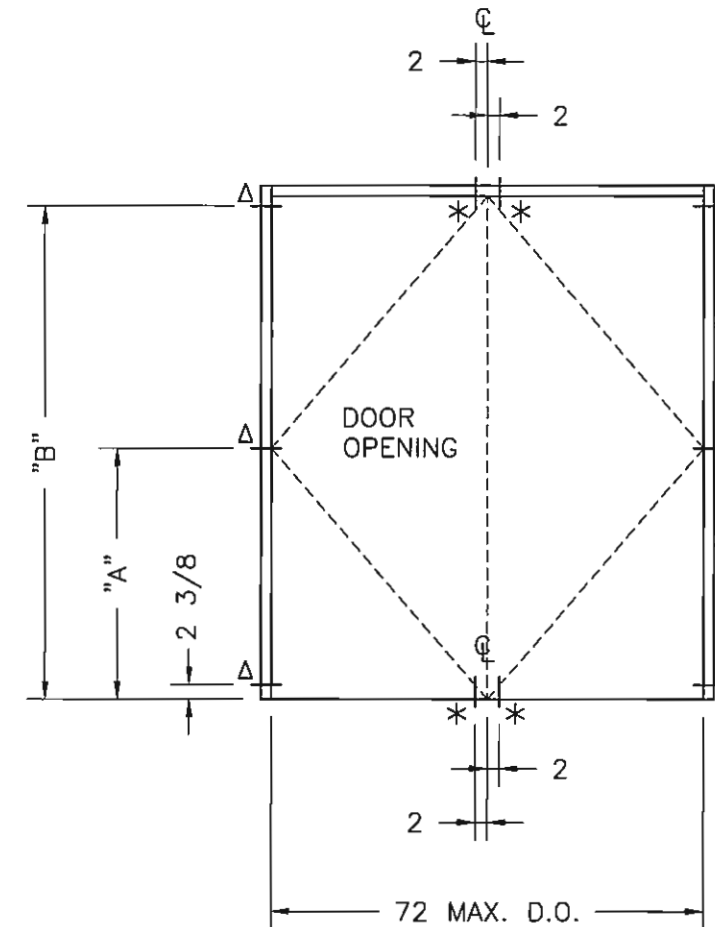
TYPICAL INSTALLATION INTO LIGHT GAUGE STEEL SUBSTRATE
