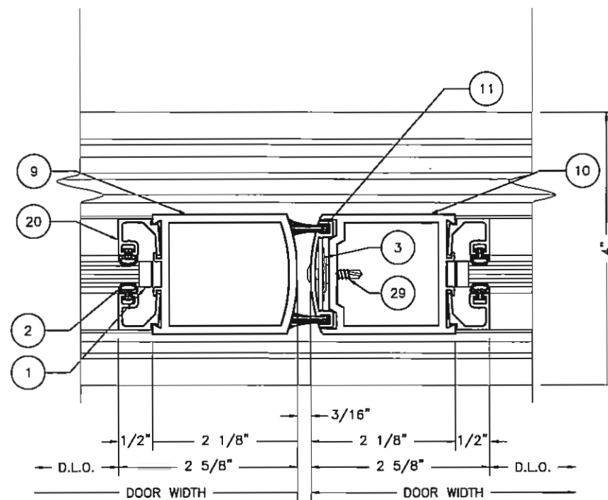
12 NS MEETING STILES 11 SCALE: 1:2
