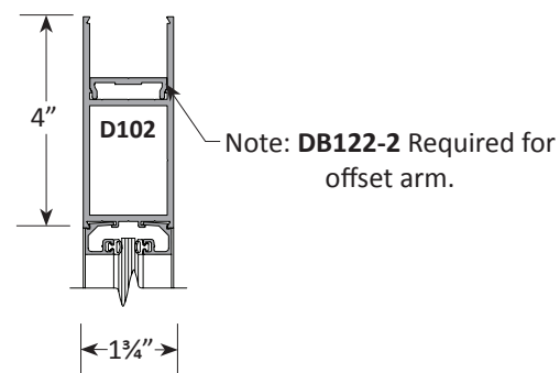
Single Acting
