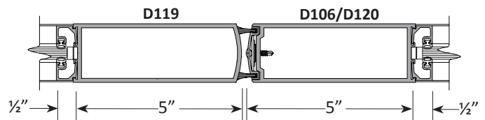
Single Acting
