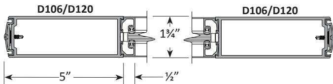
Double Acting
