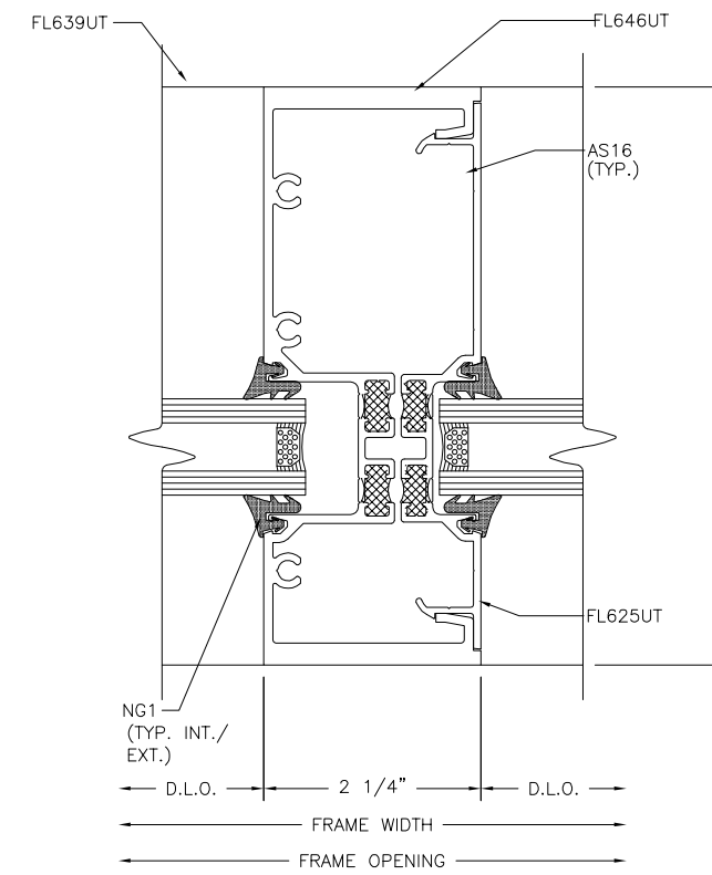
HEAVY VERTICAL
