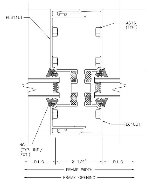
EXPANSION MULLION
