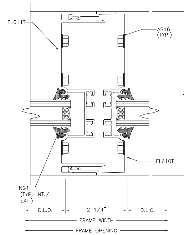
EXPANSION MULLION
