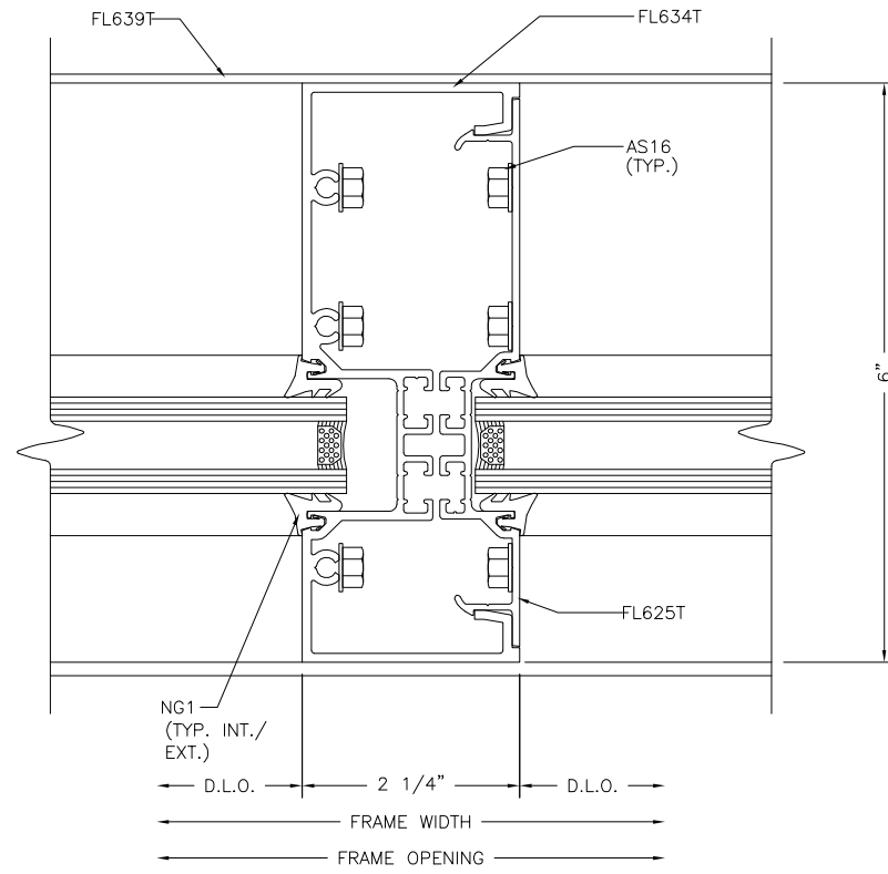
VERTICAL MULLION
