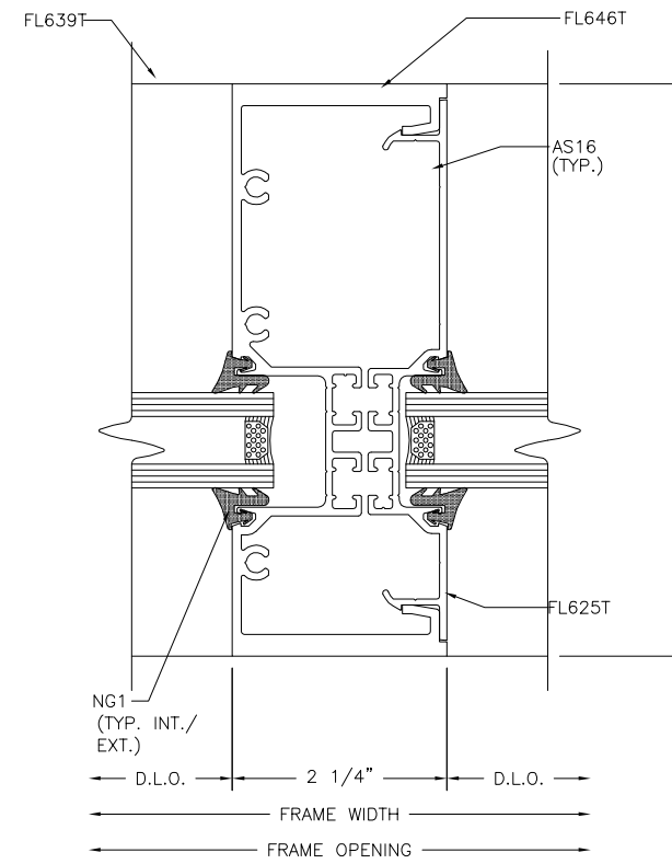
HEAVY VERTICAL
